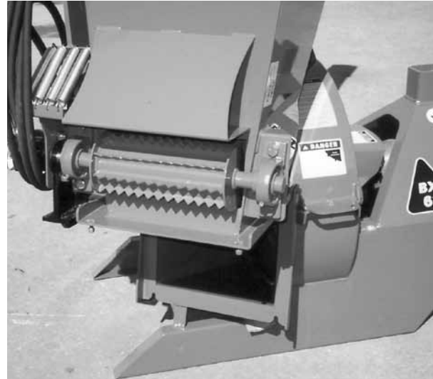
Feed Hopper
