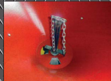
Optional chain agitator to prevent bridging of material
