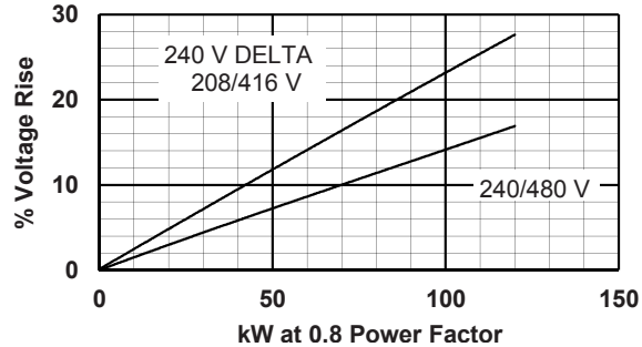
LOAD REJECTION
